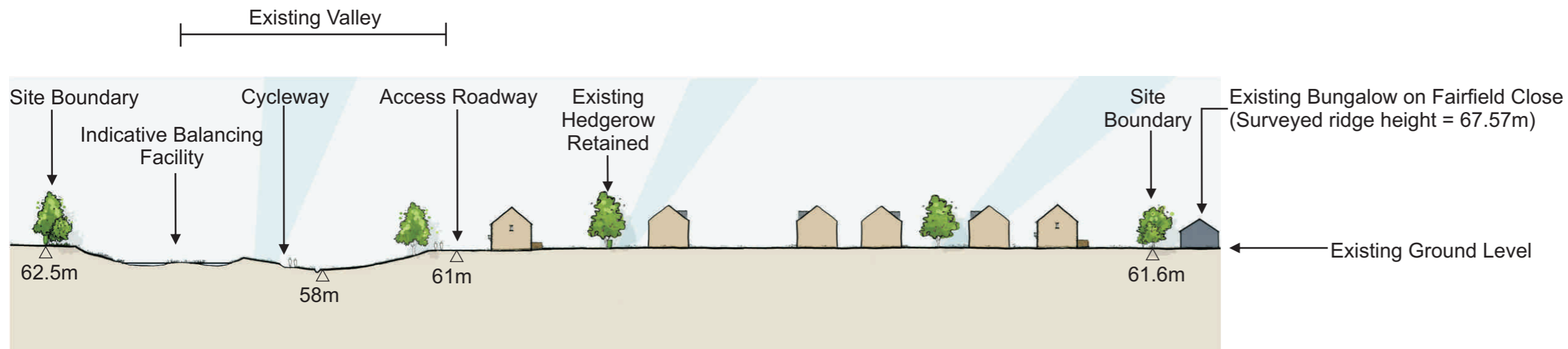
Indicative Cross Section A
