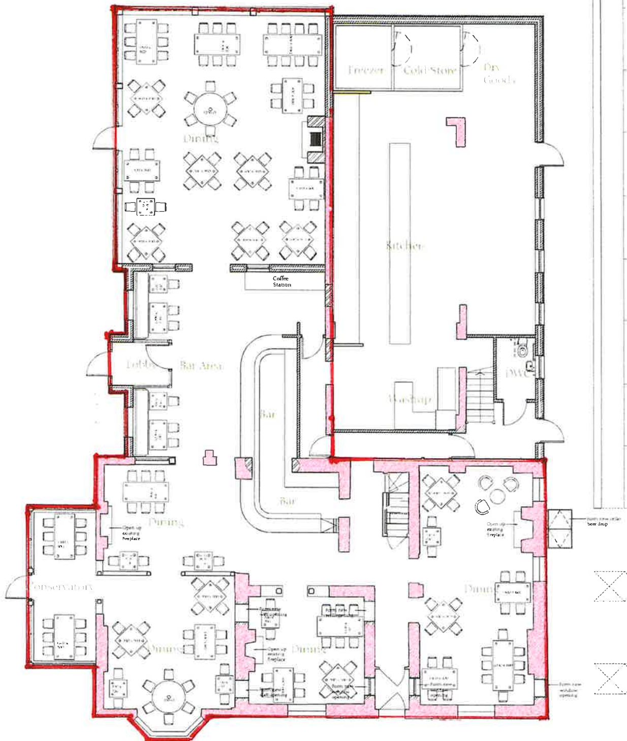
Ground Floor Plan scale 1/50 @ A1, 1/100 @ A3
