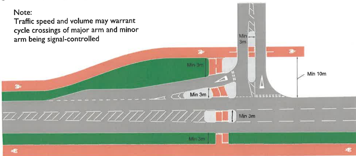
Figure 10.18: Cyclists give way on minor arm
