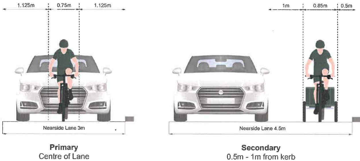
Figure 7.2: Primary and secondary riding positions
