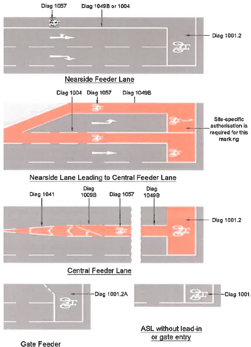
Figure 10.35: Typical arrangements for ASLs
