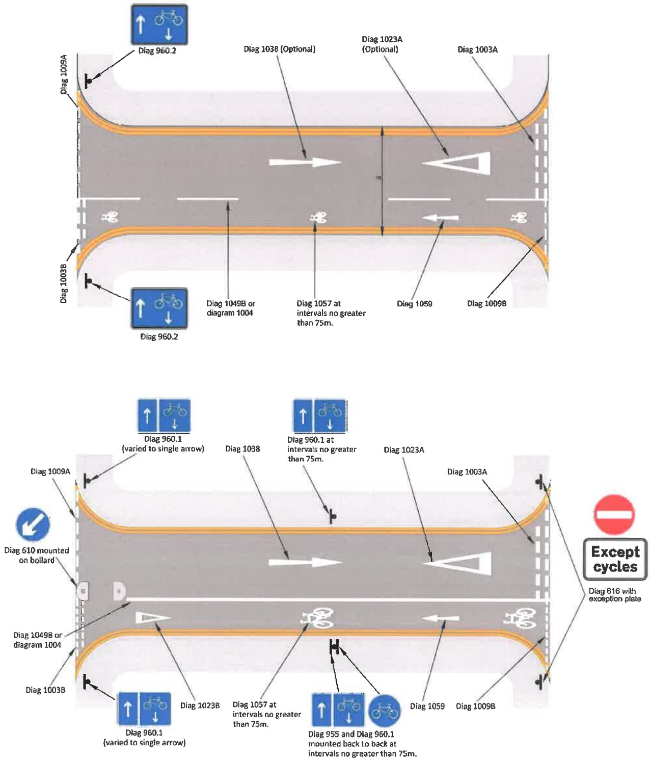
Figure 6.25: Contraflow cycle lanes
