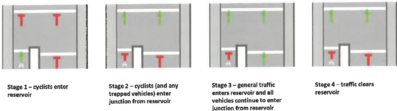
Figure 10.34: Cycle gate signal sequence
