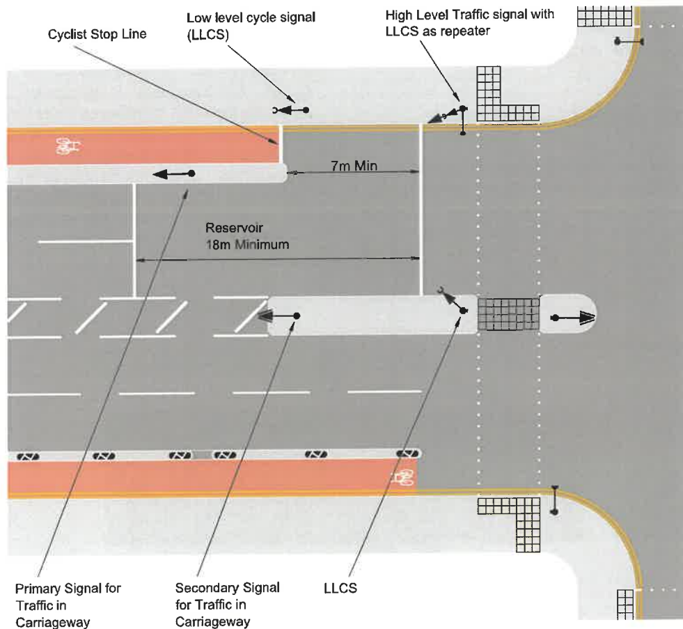
Figure 10.33: Cycle gate layout
