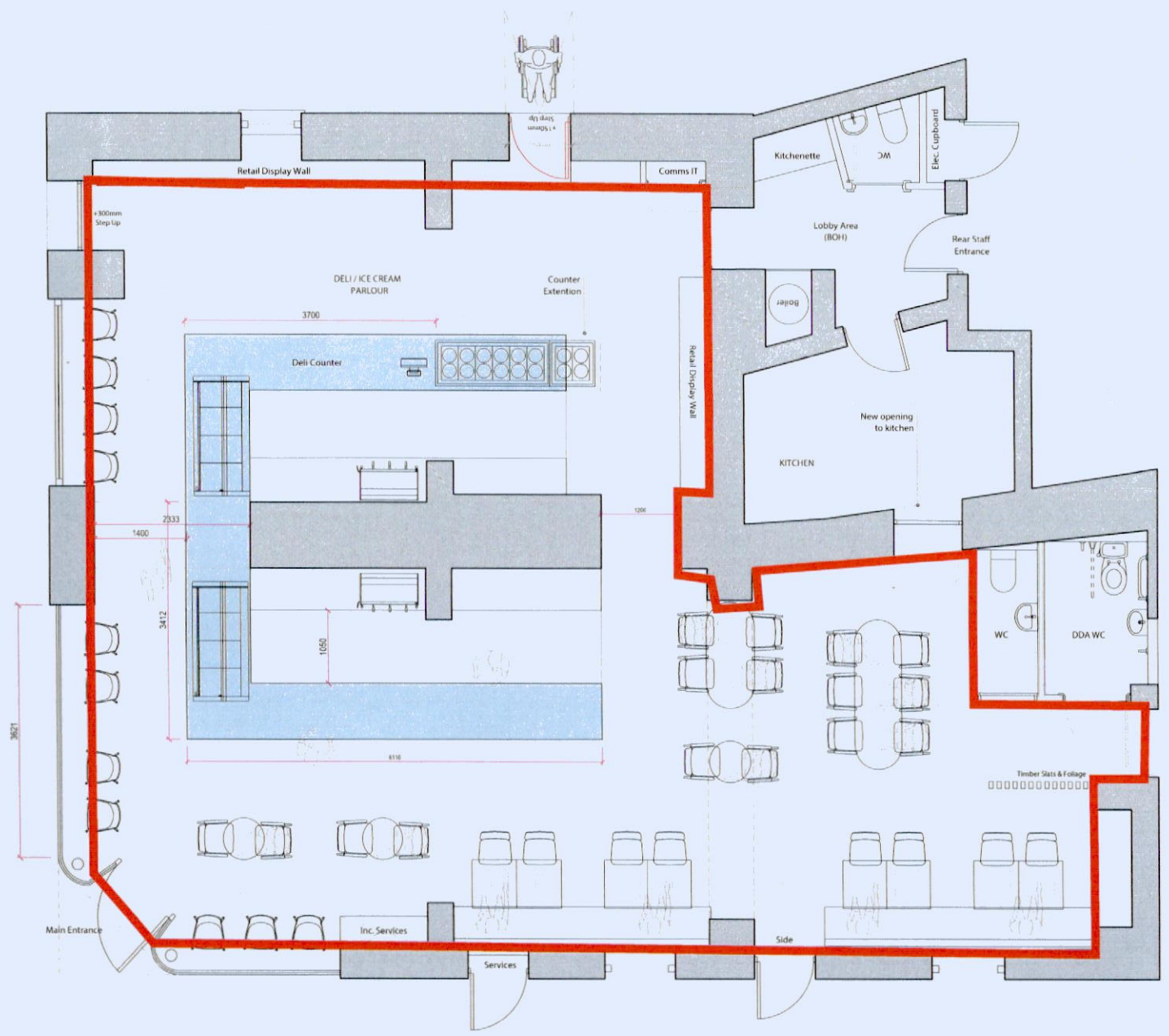
PROPOSED GENERAL ARRANGEMENT PLAN
