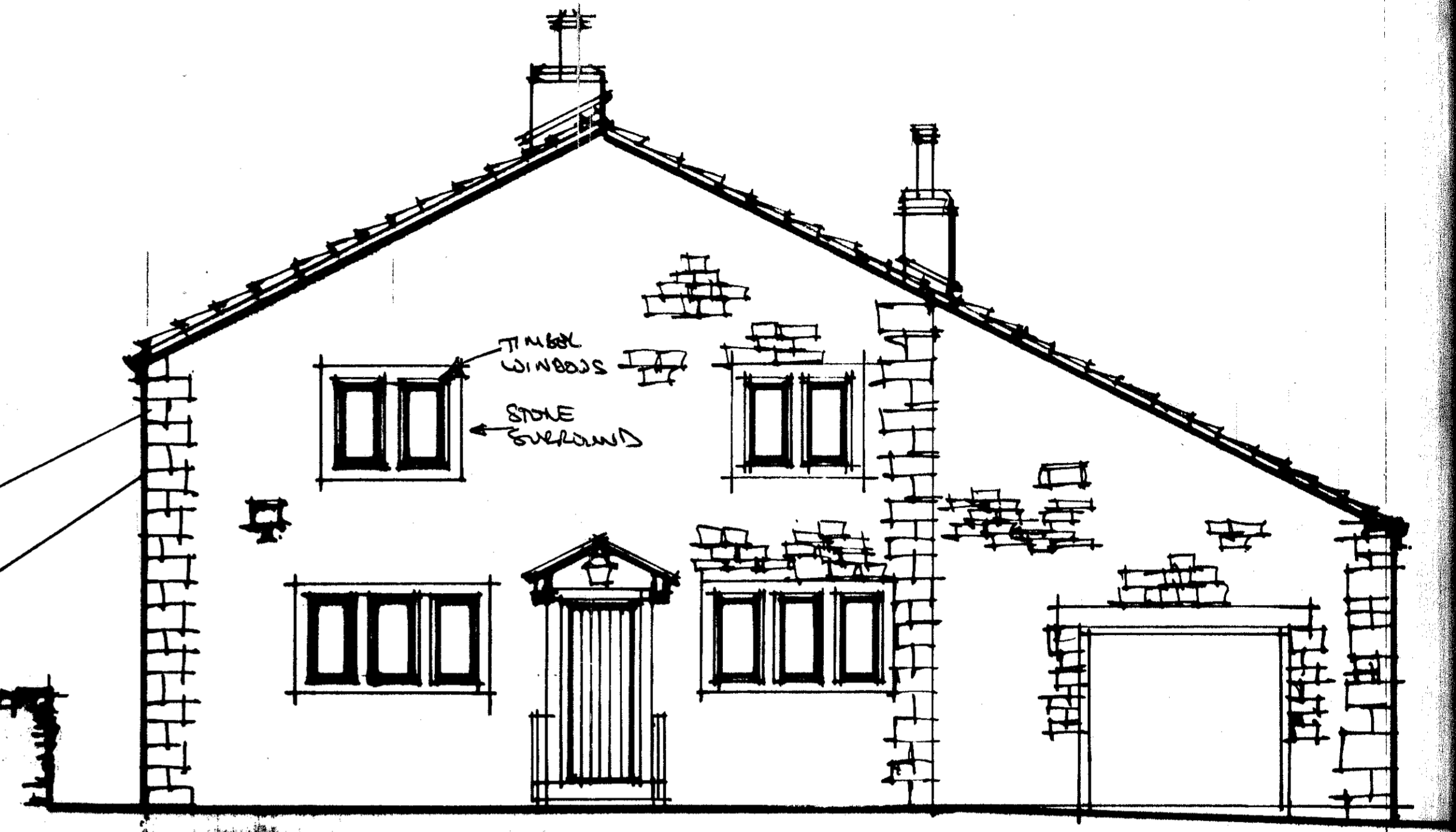
FRONT ELEVATION:
