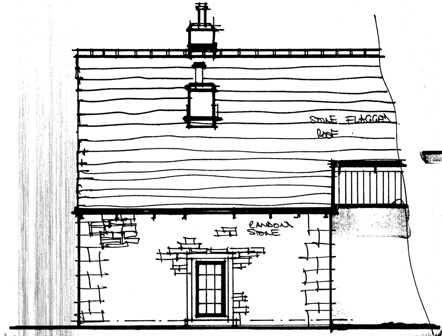
SIDE ELEVATION
